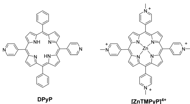
Fig. 24 Chemical structures of DPYP and [\text{ZnTMPyP}]^{4+} porphyrins.
