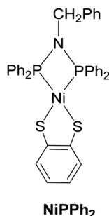
Fig. 22 Chemical structure of a mononuclear nickel catalyst ( \text{NiPPh}_2 ).
