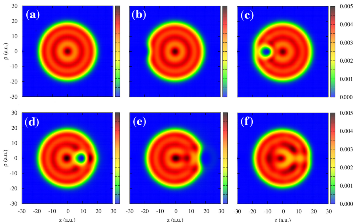
Fig. 6 Electron density of the \text{Na}_{106} cluster (radius R_{cl} = 18.93 a.u.) upon collision with antiproton. Results are shown as a function of the cylindrical ( z, \rho ) coordinates. The projectile moves with the constant velocity v = 0.3 a.u. along a straight-line trajectory following the symmetry z -axis of the system that passes through the center of the cluster. The snapshots correspond to six different antiproton positions: (a) z_p = -30 a.u., (b) z_p = -20 a.u., (c) z_p = -10 a.u., (d) z_p = 10 a.u., (e) z_p = 20 a.u., and (f) z_p = 30 a.u. The color code shows the electron density of the cluster in electrons per (a.u.) 3 .
