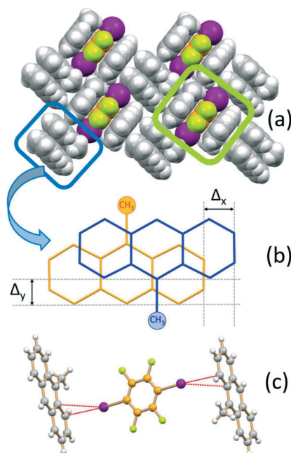
Fig. 3 Packing features of (MA)_4-I2F4 showing (a) the I2F4 molecules “sandwiched” between MA molecules (lime rectangle) and the \pi -stacked MA pairs (blue rectangle), (b) details of the head-to-tail pair arrangement ( \Delta y and \Delta x indicate the transversal and longitudinal offsets, respectively), and (c) the geometry of the I\cdots\pi interactions.
