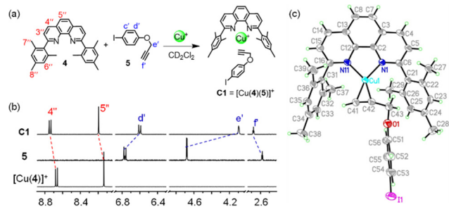
Fig. 2 (a) Formation of model complex C1 . (b) Partial ^1\text{H} NMR (400 MHz, 298 K) of [\text{Cu}(\text{4})]^+ , 5 and C1 in \text{CD}_2\text{Cl}_2 (2.5 mM). (c) X-ray crystal structure of complex C1 . Carbons are shown in light grey; H, light green; N, blue; O, red; \text{Cu}^+ , cyan and I, violet.
