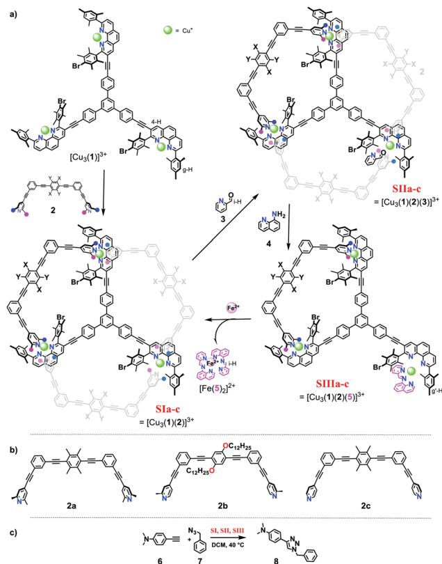
Fig. 1 (a) A three-component slider-on-deck that is modulated upon addition of external stimuli (grey: bipes in motion). (b) Molecular structure of bipes 2a–c . (c) Model reaction catalysed by slider-on-deck systems.
