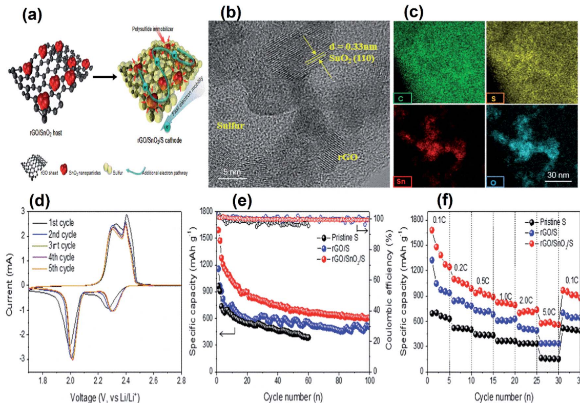
Fig. 32 Schematic representation of the rGO/SnO 2 /S cathode acting as a polysulfide immobilizer (a); HRTEM image (b) and elemental mapping (c) of the rGO/SnO 2 /S composite; cyclic voltammetry curve at 0.1 mV s -1 (d); and cycling performance (e) and rate performance (f) of the rGO/SnO 2 /S composite. 366 Adapted with permission of Elsevier.
