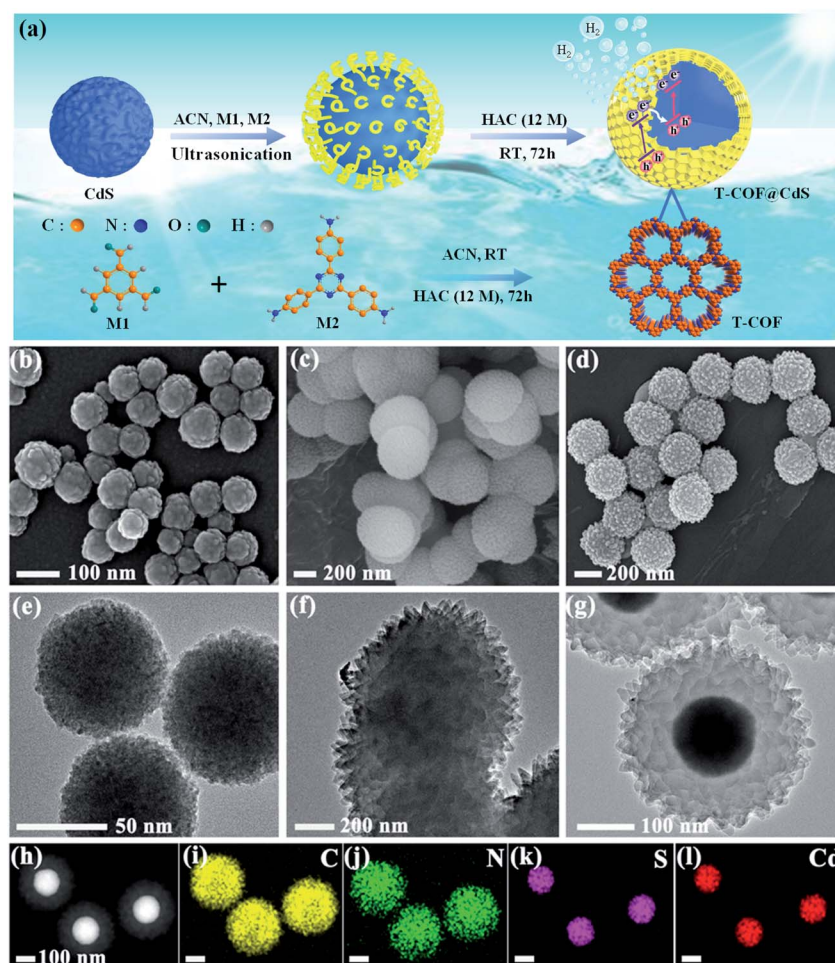
Fig. 1 (a) Schematic illustration of the preparation of T-COF@ \text{CdS} . SEM images of (b) \text{CdS} , (c) T-COF, and (d) T-COF@ \text{CdS} -3. TEM images of (e) \text{CdS} , (f) T-COF, and (g) T-COF@ \text{CdS} -3. (h) The HAADF-TEM image of T-COF@ \text{CdS} -3. (i–l) EDX elemental mapping of T-COF@ \text{CdS} -3.
