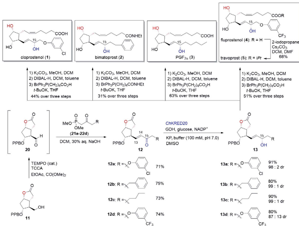
Fig. 5 Completion of the chemoenzymatic total synthesis of cloprostenol (1), bimatoprost (2), PGF_{2\alpha} (3), fluprostenol (4), and travoprost (5).
