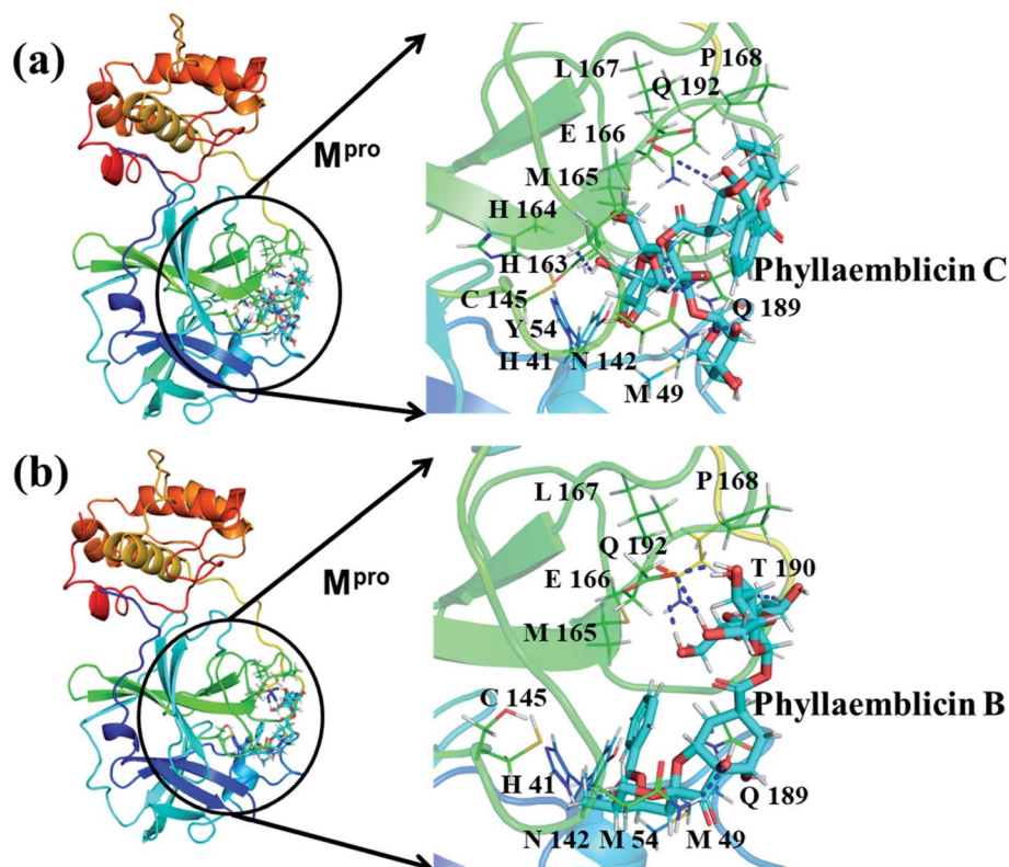
Fig. 3 SARS-CoV-2 M^{pro} in complex with phytochemicals: the molecular interactions of phyllaemblicin C with the M^{pro} protein (a) and phyllaemblicin B with the M^{pro} protein (b). The protein is represented as cartoon, the interacting amino acid residues are shown as lines and the hydrogen bonding interactions are represented using blue dotted lines. The ligand (phytochemical) is represented as cyan sticks.
