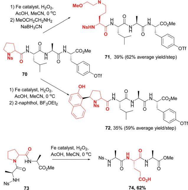
Scheme 18 Use of proline customizable units by White et al. 12
