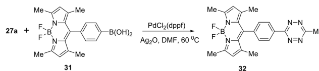
Scheme 13 Synthesis of BODIPY-tetrazine conjugate 32 .
