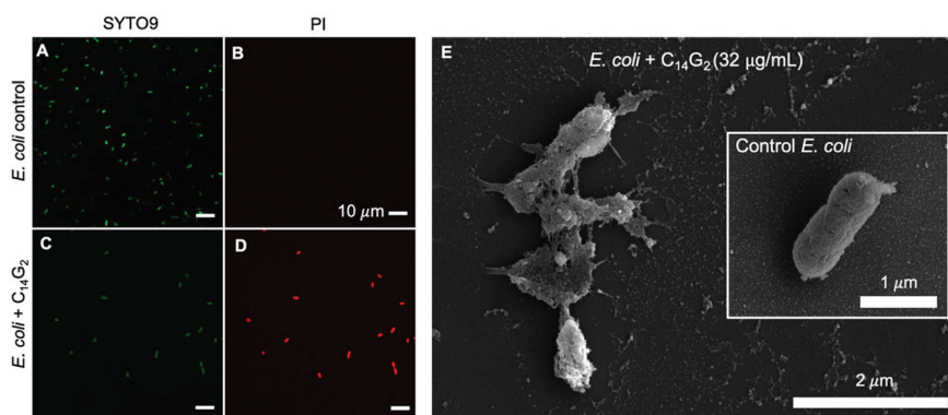
Fig. 1 Confocal laser scanning microscopy images of (A and B) E. coli in PBS and (C and D) E. coli exposed to C_{14}G_2 at 32\ \mu\text{g mL}^{-1} and (E) Scanning Electron Microscopy (SEM) images of E. coli exposed to C_{14}G_2 at 32\ \mu\text{g mL}^{-1} compared to (inset) E. coli alone, both after fixation.
