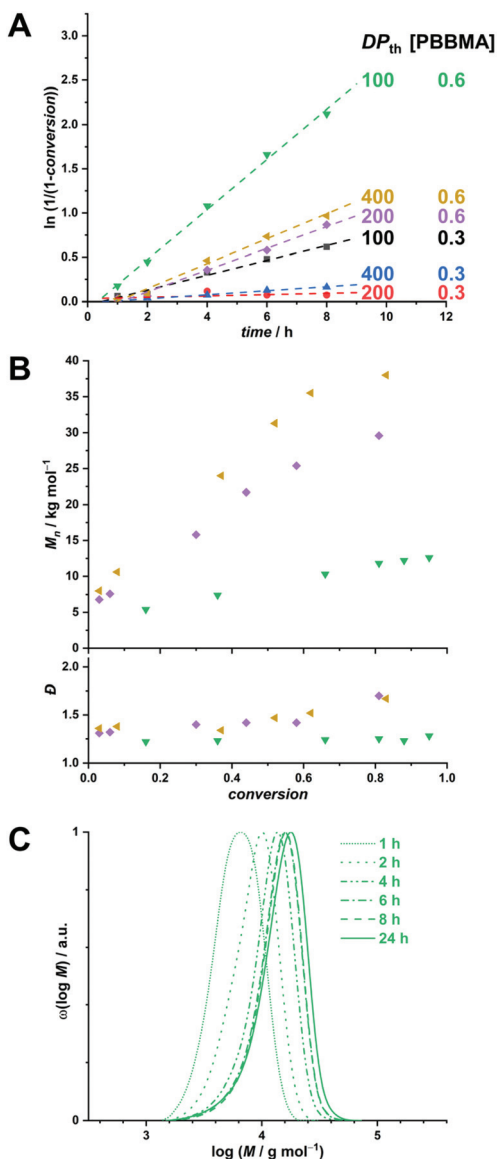
Fig. 1 RAFT solution polymerization of PBBMA in DMAc at 70 °C. (A) First-order kinetic plots for various [PBBMA] and DP th . Dashed lines correspond to linear fits. (B) Evolution of number-average molar mass (top) and dispersity (bottom) with PBBMA conversion for [PBBMA] = 0.6 M at various DP th . (C) Size-exclusion chromatograms of polymers obtained at different times for [PBBMA] = 0.6 M and DP th = 100.
