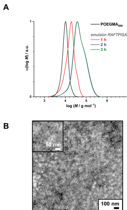
Fig. 2 (A) Size-exclusion chromatograms of polymers obtained by PBBMA emulsion RAFTPISA in water/ethanol 3 : 1 vol/vol at 70 °C with POEGMA 500 at DP th = 100, and 20 wt% solids content (entry 4 from Table S2 † ). (B) Transmission electron micrograph of nanoparticles obtained in the conditions mentioned above, after 2 h.
