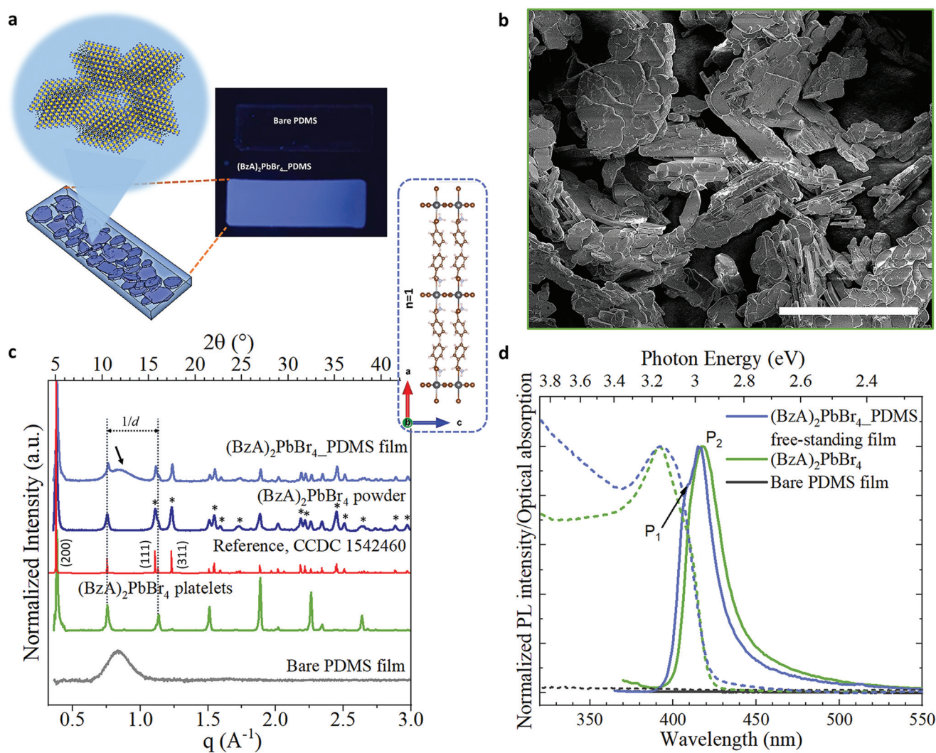
Fig. 1 (a) Scheme showing the atomic layered structure of the (\text{BzA})_2\text{PbBr}_4 platelets nucleated in situ in the PDMS by injecting the amine in the mixture of PDMS, \text{PbBr}_2 , \text{HBr} and acetone. The photograph displays the resulting blue-emitting film under UV lamp irradiation. (b) SEM images of the platelets without PDMS and deposited on a Si substrate. Scale bar: 50 \mu\text{m} . (c and d) XRD patterns (c) and emission spectra and optical absorption (d) collected from bare PDMS film (grey), ensembles of the perovskite platelets (green), powder sample of platelets, and free-standing film of 2D layered perovskite–PDMS (blue). In red, the reference from ref. 34. In (c): the inset displays the b-view of the orthorhombic unit cell of (\text{BzA})_2\text{PbBr}_4 crystals from ref. 34; the dotted lines indicate the highly intense periodic diffraction peaks of the platelet ensembles from their preferential crystal orientation parallel to the substrate, which is partially retained in the films; the black arrow highlights the broad peak from the PDMS in the composite films and the asterisks indicate the most intense Bragg reflections associated to different diffraction planes.
