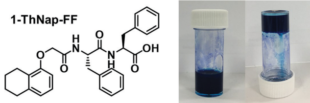
Fig. 6 The chemical structure of 1-ThNap-FF and photographs of the blend (^1\text{PrNH})_2\text{NDI-V} ( 5 \text{ mg mL}^{-1} ) and 1-ThNap-FF ( 5 \text{ mg mL}^{-1} ) hydrogel.
