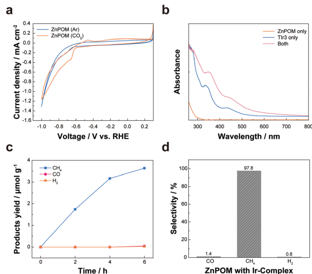
Fig. 2 Photochemical \text{CO}_2\text{RR} using ZnPOM as a catalyst and TlIr3 as a photosensitizer. (a) CV analysis of ZnPOM in 0.1 M \text{KHCO}_3 saturated with Ar or \text{CO}_2 gas. (b) UV/visible absorbance spectra of each component and both in 0.1 M \text{KHCO}_3 . (c) Production and (d) selectivity of various chemicals upon photochemical \text{CO}_2\text{RR} using 30 \mu\text{M} ZnPOM, 0.1 mM TlIr3, and 0.05 M \text{Na}_2\text{SO}_3 under visible light irradiation. The selectivity of each product was calculated after 6 h of photochemical \text{CO}_2\text{RR} by considering the number of electrons required to produce each.
