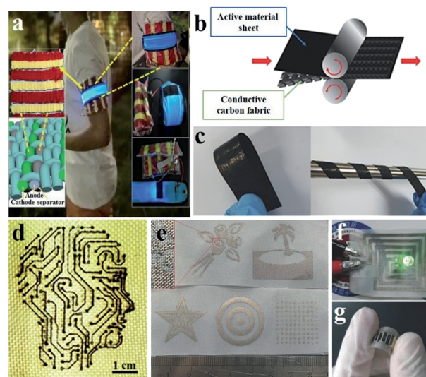
Fig. 8 (a) Batteries knitted into a sweater (the yellow arrow is pointing) and used as power sources lighting the LED bands. Reproduced with permission. 135 Copyright 2020, Wiley-VCH. (b) Schematic demonstration of the preparation process of the electrode. (c) Photograph of prepared flexible electrodes. Reproduced with permission. 136 Copyright 2018, Wiley-VCH. (d) Photograph of LiG patterned into a human side face shape. Reproduced with permission. 18 Copyright 2020, American Chemical Society. (e) Different conductive patterns drawing on two polyester fabrics. (f) The DC power source powered the green LED through the textile conductive circuit. (g) Photograph of fabricated textile MSC. Reproduced with permission. 137 Copyright 2016, Wiley-VCH.
