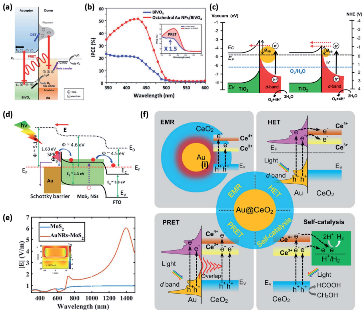
Fig. 15 (a) Energy band diagram of the BiVO 4 photoanode with an octahedral Au NP that shows the HET (DET) and PRET mechanisms. (b) IPCE spectra of BiVO 4 and octahedral Au NP/BiVO 4 photoanodes at 1.23 V vs. RHE. (a) and (b) are reprinted from ref. 158, copyright 2017, with permission from Wiley-VCH. (c) Schematic of the energy band diagram for a Au NP/TiO 2 nanotube array-photoelectrode under visible light illumination that shows the mechanism for the hot electron mediated OER. Reprinted from ref. 163, copyright 2018, with permission from the Royal Society of Chemistry. (d) Energy band diagram of the Au-MoS 2 heterostructure with formation of a Schottky barrier. (e) Calculated electric field intensity as a function of wavelength. The inset shows the electric field distribution at 1405 nm. (d) and (e) are reprinted from ref. 168, copyright 2019, with permission from the Royal Society of Chemistry. (f) Possible mechanisms for the HER in a Au@CeO 2 core-shell photocatalyst under visible light illumination. Reprinted from ref. 171, copyright 2021, with permission from Elsevier.
