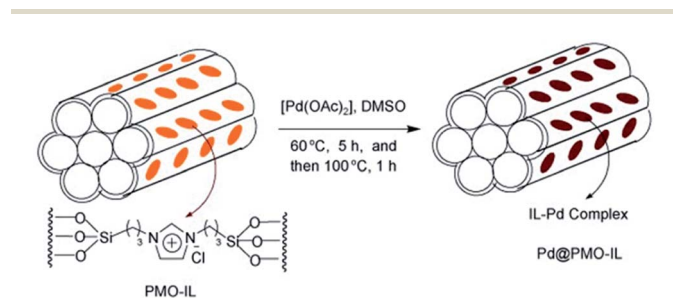
Fig. 30 The preparation of the Pd@PMO-IL catalyst. 181 Reproduced with permission. 181 Copyright 2010, John Wiley & Sons.
