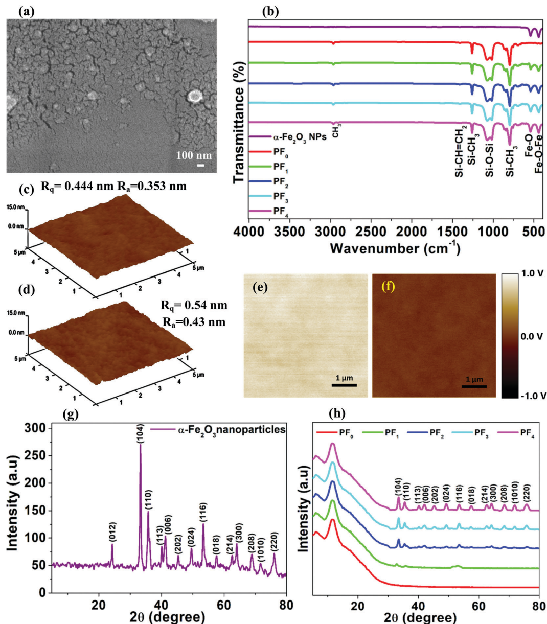
Fig. 2 (a) FESEM view of the PDMS film and (b) FTIR spectra of \alpha -Fe 2 O 3 NPs, PDMS, and PDMS@ \alpha -Fe 2 O 3 NP composites; AFM images (three-dimensional) of the (c) PDMS film and (d) PDMS@ \alpha -Fe 2 O 3 NP composite film; KPFM images of (e) PDMS film and (f) PDMS@ \alpha -Fe 2 O 3 NP composite film. XRD plots of (g) \alpha -Fe 2 O 3 nanoparticles and (h) PDMS@ \alpha -Fe 2 O 3 NP composites.
