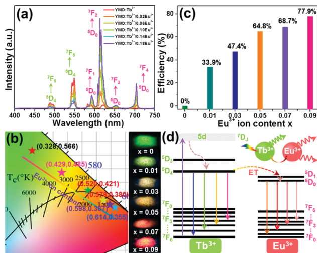
Fig. 3 (a) Emission spectra and (b) CIE chromaticity diagram and optical images of YMO:Tb 3+ /2xEu 3+ (0 ≤ x ≤ 0.09) NTE microparticles. (c) ET efficiency as a function of Eu 3+ ion content. (d) Simplified energy level diagram describing the ET process in the YMO:Tb 3+ /2xEu 3+ NTE microparticles.
