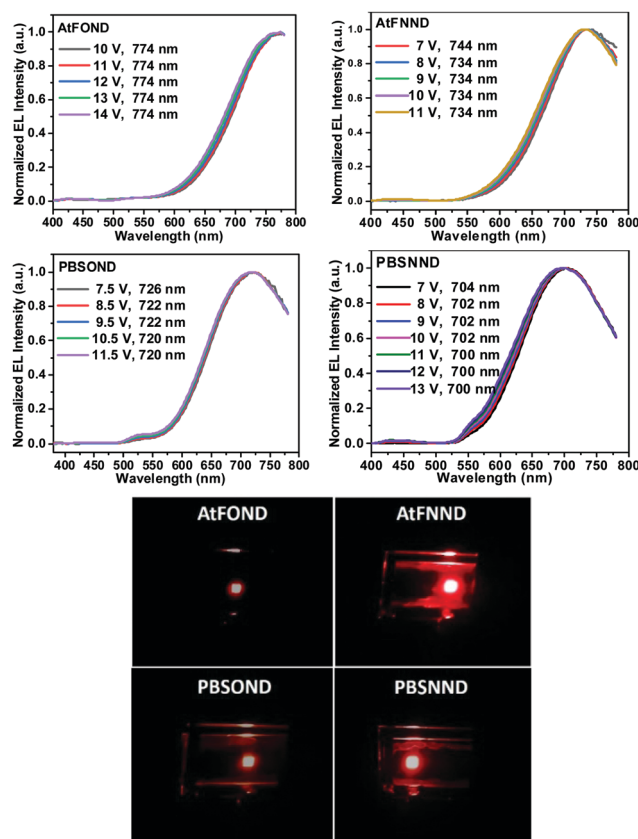
Fig. 8 Top figures: intensity normalized EL spectra AtFOND, AtFNND, PBSOND, and PBSNNND NIR OLEDs at varied voltage. Bottom figures: corresponding photographs of each device at \sim 4 – 6 V.
