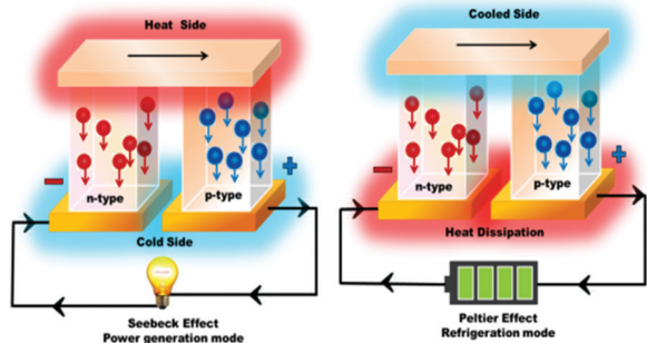
Fig. 2 Schematic of the thermoelectric and Peltier cooling modules.
