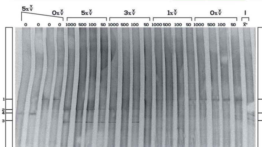
Fig. 3 (A) Maximum likelihood inferred 16S rRNA phylogenetic reconstruction from excised DGGE bands. Black circles correspond to a 1000 bootstrap, SH-aLRT \geq 80\% and ultra-fast bootstrap \geq 95\% . (B) DGGE fingerprinting image from the BMP sludge with anaerobic treatment (0% v/v), microaerobic 1% v/v O_2 , 3% v/v O_2 , 5% v/v O_2 and inoculum (I). Numbers on the top of each column (0, 50, 100, 500 and 1000 ppm) correspond to PDMS concentrations per treatment, X^* corresponds to the PDMS concentration inferred from literature. Dominant DGGE bands correspond to the chart at the bottom and the phylogenetic reconstruction.
