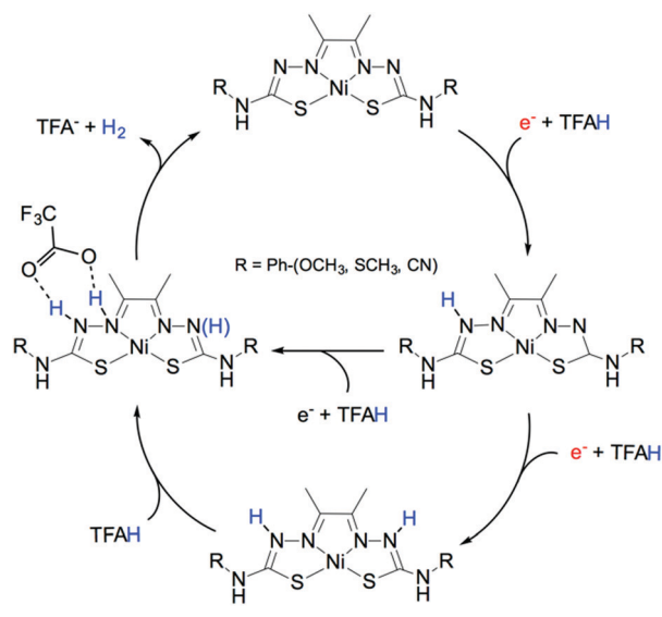
Fig. 18 DFT computed reaction mechanism for hydrogen evolution mediated by a molecular catalyst highlighting the influence of the proton source on the preferable pathway. Adapted with permission from ref. 309. Published by The Royal Society of Chemistry.
