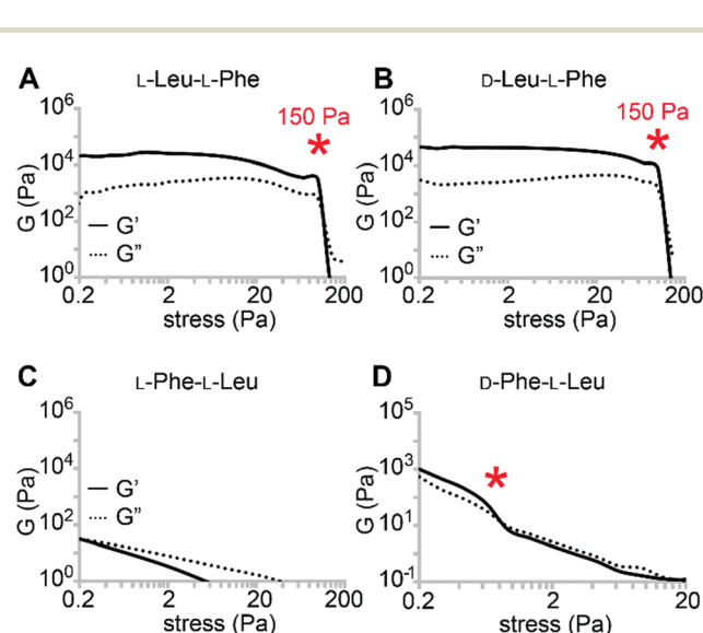
Fig. 2 Oscillatory rheology stress sweeps for the four dipeptides. Red stars mark gel-to-sol transitions.
