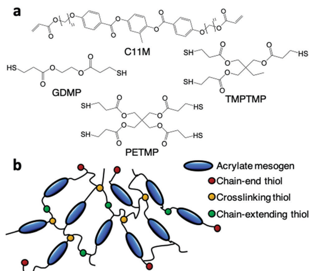
Fig. 1 (a) The diacrylate liquid crystal monomer C11M was copolymerized with thiol monomers GDMP (difunctional), TMPTMP (trifunctional), and PETMP (tetrafunctional). (b) Thiols in the crosslinked system may participate in four ways: as chain ends, crosslinkers (for trifunctional or greater), or chain-extenders.
