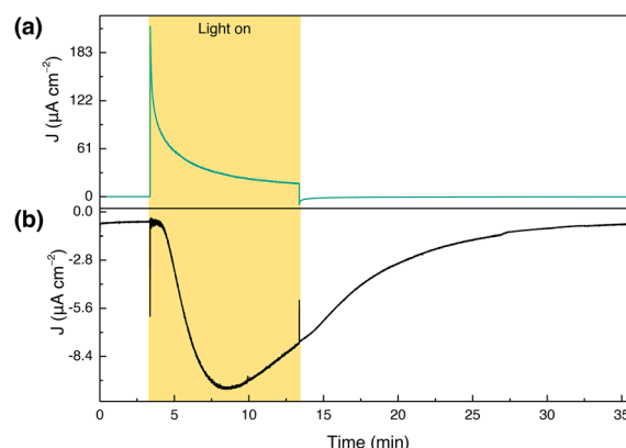
Fig. 4 Collector-generator experiment for a \text{TiCl}_4\text{-mTiO}_2\text{[DPP-Ru/CDCA]} electrode prepared by immobilisation in MeOH solution (0.1 mM DPP-Ru and 20 mM CDCA). Conditions: NaOAc buffer (0.1 M, pH 5.6) with \text{NaClO}_4 (0.4 M), 100 \text{ mW cm}^{-2} , AM 1.5G, \lambda > 420 \text{ nm} , \text{N}_2 purged, room temperature. (a) Chronoamperometry photocurrent trace of the generator with an applied potential of +0.2 vs. NHE. (b) Chronoamperometry current trace of the collector with an applied potential of -0.6 vs. NHE.
