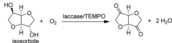
Scheme 12 Laccase/TEMPO catalysed oxidations of alcohols.
