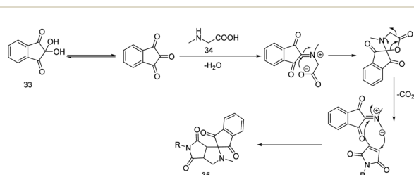
Scheme 11 Proposed mechanism for the formation of dihydro-2' H -spiro[indene-2,1'-pyrrolo[3,4- c ]pyrrole]-tetraone derivatives. This figure has been reproduced from ref. 20 with permission from Elsevier, copyright 2020
