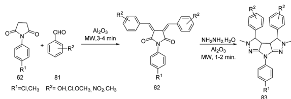
Scheme 26 Synthesis of hexahydro-2 H -pyrrolo[2,3- c :5,4- c' ]dipyrroles from chalcone through a microwave mediated protocol.
