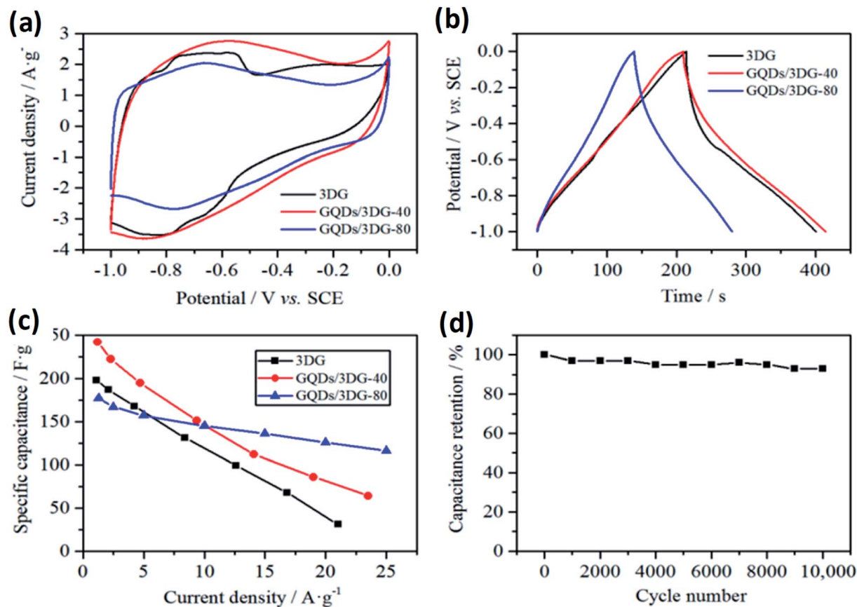
Fig. 18 (a) Cyclic voltammety curve at a scan rate of 10 mV s -1 (b) charge/discharge curves at different current densities with different compositions, respectively (c) specific capacitance versus current densities and (d) cycling stability at a current density of 24 A g -1 for the composite material. Adapted from ref. 183, copyright 2019, MDPI publications.
