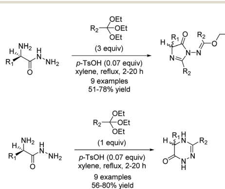
Scheme 9 Jasiak and co-workers' synthesis of imidazol-4-ones from optically active \alpha -aminocarboxylic acid hydrazides.
