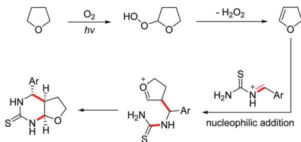
Scheme 37
