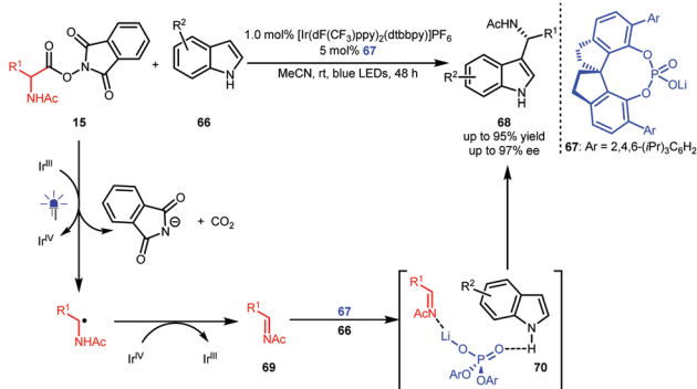
Scheme 16 Enantioselective Friedel–Crafts reaction.
