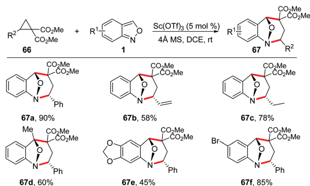
Scheme 23 [4 + 3]-annulation reaction between cyclopropane 1,1-diesters and anthranils.
