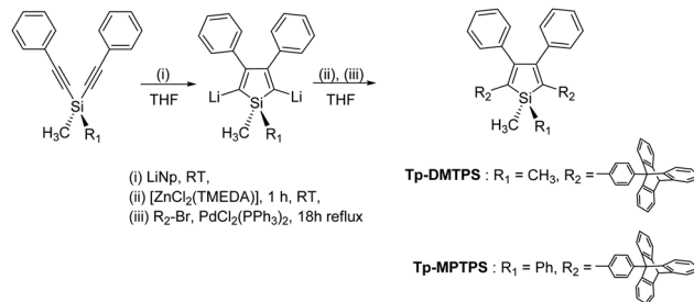
Scheme 1 Synthetic route to Tp-DMTIPS and Tp-MPTPS (see more details in ESI†).
