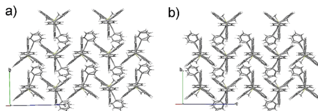
Fig. 2 Views of the crystal packing of Tp-DMTIPS showing the triptycene paving in the bc plane for (a) R -conformers and (b) L -conformers.
