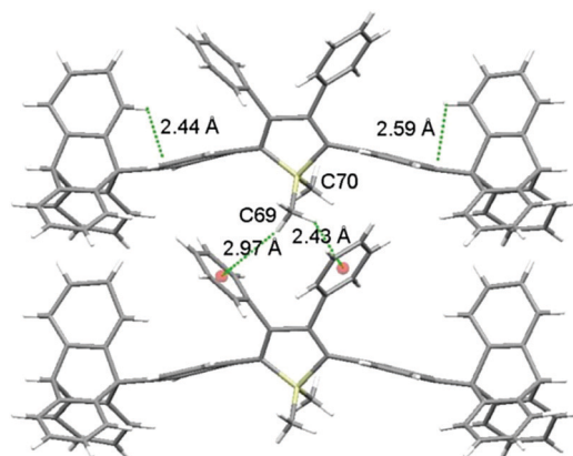
Fig. 3 View of the R -conformers of Tp-DMTIPS in the ab plane showing the methyl C69 nestling between the aromatic rings. Intra and intermolecular CH/ \pi interactions are marked with green dotted lines.
