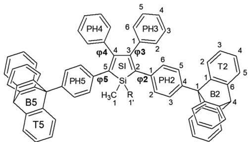
Fig. 1 Labelling scheme for Tp-DMTIPS ( R1' = \text{Me} ) and Tp-MPTPS ( R1' = \text{Ph} ).
