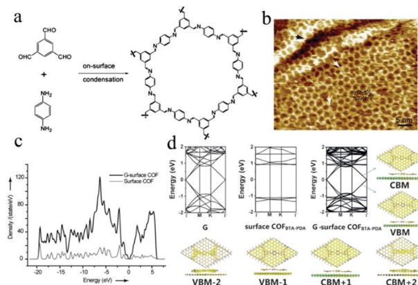
Fig. 13 (a) Reaction scheme of Schiff base condensation between benzene-1,3,5-tricarbaldehyde (BTA) and p -phenylenediamine (PDA) into hexagonal 2D surface COF_{BTA-PDA} . (b) STM image of surface COF_{BTA-PDA} on SLG-copper (single layer graphene grown by CVD on copper). A “5 + 7” defect is highlighted by an overlaid schematic model and two typical domain boundaries are marked by the white arrows. A perfect chain of hexagons crossing the step edge of copper is marked by a black arrow. (c) Density of states of G-surface COF_{BTA-PDA} (the surface of COF_{BTA-PDA} –graphene complex) and surface COF_{BTA-PDA} (Fermi level is set at 0 eV). (d) The band structures of graphene, surface COF_{BTA-PDA} , G-surface COF_{BTA-PDA} and the decomposed charge density of G-surface COF_{BTA-PDA} near the Fermi level (Fermi level is set at 0 eV). Copyright 2014, Angewandte Chemie International Edition. 46
