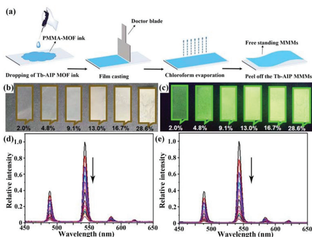
Fig. 23 (a) The preparation process of Tb-AIP MMMs. Images of Tb-AIP MMMs by varying the additional amounts of MOF powders (b) under natural light and (c) UV lamp at 365 nm. Emission spectra of Tb-AIP MMMs upon increasing concentrations of (d) NFZ and (e) NFT. Reproduced from ref. 127 with permission from Elsevier.
