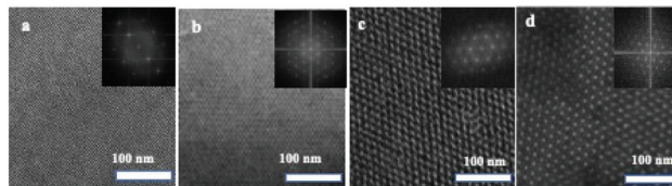
Fig. 2 TEM images of thin fcc supracrystals of Ag nanocrystals coated with oleylamine ( C_{18}\text{-NH}_2 ) with different average diameters: (a) 2.2 nm; (b) 4.1 nm; (c) 8.7 nm; and (d) 12.9 nm. Inset: Fourier transform of the TEM image.
