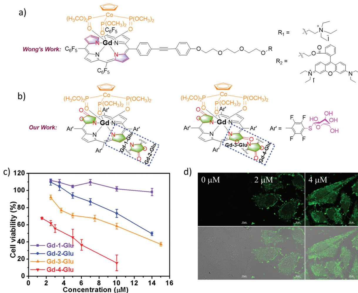
Fig. 15 (a) Chemical structure of Wong's work on the design of Gd theranostic agents. (b) Chemical structure of our work on the design of Gd theranostic agents. (c) Photocytotoxicity of Gd -1–4-Glu toward HeLa cells by using a CCK-8 assay under different wavelengths of light irradiation at 600–700 nm with the same dose of light ( 6.5 \text{ mW cm}^{-2} ) for 30 min, and then cultured in the dark for another 24 h. (d) H2DCFDA fluorescence images of HeLa cells under different drug doses of Gd -2-Glu; 0–2 \mu M Gd -2-Glu in the dark for 24 h, 10 \mu M H2DCFDA for 30 min, then irradiated with visible light (400–700 nm, 6.5 \text{ mW cm}^{-2} ) for 30 min. Reproduced with permission from ref. 62. Copyright 2016 Wiley-VCH.
