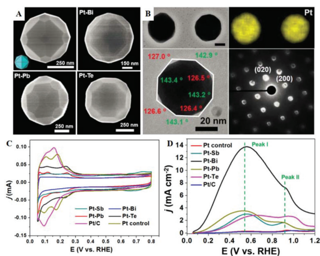
Fig. 8 (A) Representative SEM images of THH Pt, and Pt particles synthesized through Bi, Pb, and Te modification. (B) STEM images, EDS elemental maps, TEM images, and the corresponding diffraction patterns of the PtBi particles. (C) CVs of THH-shaped Pt-M (M = Sb, Bi, Pb, or Te) catalysts, Pt control sample, and commercial Pt/C catalyst in Ar-saturated 0.5 M H 2 SO 4 solution. (D) Polarization curves of formic acid oxidation for different catalysts. Reproduced with permission from ref. 138. Copyright 2019, American Association for the Advancement of Science.
