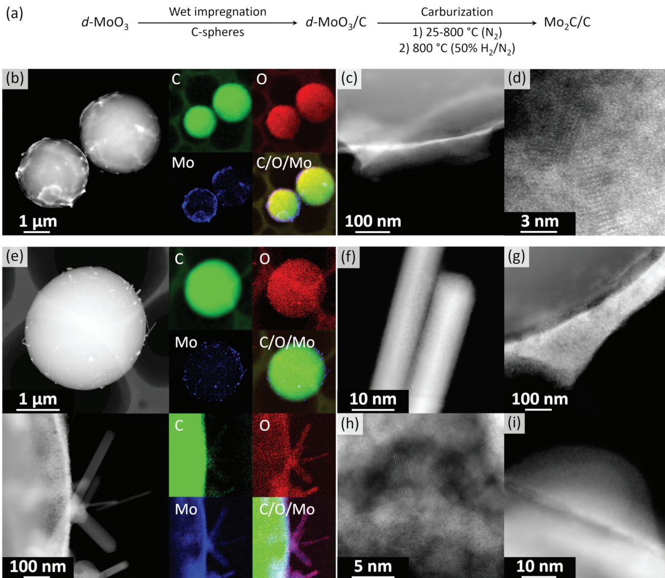
Fig. 1 (a) Synthesis of \beta\text{-Mo}_2\text{C}/\text{C} from delaminated \text{MoO}_3 films; (b) HAADF-STEM images and EDX maps of d\text{-MoO}_3/\text{C} ; (c) and (d) HR-STEM images of d\text{-MoO}_3/\text{C} ; (e) HAADF-STEM images and EDX maps of \beta\text{-Mo}_2\text{C}/\text{C} ; and (f)–(i) HR-STEM images of different morphologies decorating the surface of carbon spheres in \beta\text{-Mo}_2\text{C}/\text{C} .
