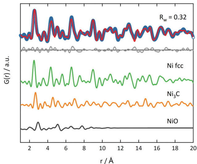
Fig. 8 PDF refinement of Ni(BDC)(PNO) decomposed at 375 °C in He with three phases ( \text{Ni}_{\text{fcc}} , \text{Ni}_3\text{C} and NiO). Blue open circles represent the experimental PDF and red line the calculated PDF. The grey line in the offset shows the difference between experimental and calculated PDF.
