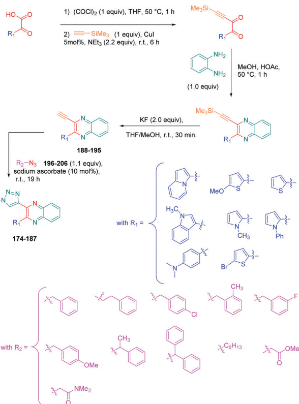
Scheme 18 One pot process for synthesis of quinoxalines 174–187 .
