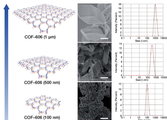
Fig. 29 COF-606 with different particle sizes measured by SEM and DLS. Scale bar: 500 nm. Adapted with permission. 198 Copyright 2020, Elsevier Inc.
