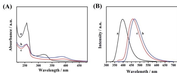
Fig. 5 (A) UV-vis absorption and (B) photoluminescence spectra of CDs-1 (a), CDs-2 (b), and CDs-3 (c).
