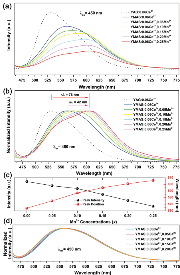
Fig. 7 (a) PL spectra and (b) normalized PL spectra of YMAS:0.06-Ce 3+ , yMn 2+ (y = 0–0.25) excited at 450 nm. (c) The variation of peak intensity and peak position with Mn 2+ concentration. (d) Normalized PL spectra of YMAS:0.06Ce 3+ , zCa 2+ (z = 0–0.20) excited at 450 nm.
