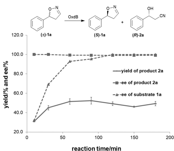
Fig. 2 Time course of the asymmetric ring-opening of 5-phenyl-4,5-dihydroisoxazole using Oxd B. The reactions were performed on a 500 \mu\text{L} scale using 100 mM KPB buffer (pH 6.0), 1 U Oxd B, 20 mM 5-phenyl-4,5-dihydroisoxazole, 0.05 mM FMN, and 1 mM \text{Na}_2\text{S}_2\text{O}_5 at 30 ^\circ\text{C} . The yield and ee were determined using chiral HPLC ( n = 2 ).
