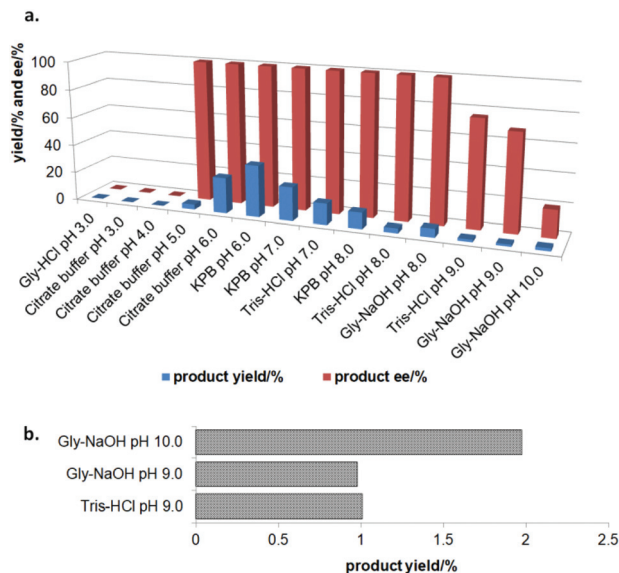
Fig. 1 (a) The pH effect on the activity of Oxd B in the catalytic asymmetric ring-opening of 5-phenyl-4,5-dihydroisoxazole. The reactions were performed on a 500 \mu\text{L} scale using 100 mM buffer (pH 3.0–10.0), 1 U Oxd-B, 20 mM 5-phenyl-4,5-dihydroisoxazole, 0.05 mM FMN, and 1 mM \text{Na}_2\text{S}_2\text{O}_5 at 30 ^\circ\text{C} for 30 min. The buffer solutions used were Gly-HCl (pH 3.0), Citrate-buffer (pH 3.0, 4.0, 5.0, and 6.0), KPB (pH 6.0, 7.0, and 8.0), Tris-HCl (pH 7.0, 8.0, and 9.0), and Gly-NaOH (pH 8.0, 9.0, and 10.0). (b) The control experiments were carried out without Oxd B at pH 9.0 and pH 10.0. The yield and ee were determined using chiral HPLC ( n = 2 ).
