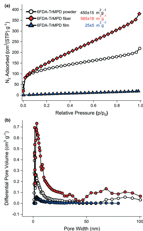
Fig. 4 a) Nitrogen adsorption isotherms measured at -196 \text{ °C} up to 1 bar, b) NLDFT-derived pore size distributions of the 6FDA-TrMPD polymer powder, the nanofibrous mat and the film.
