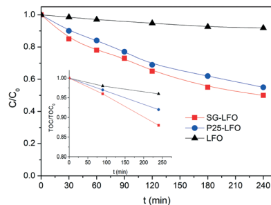
Fig. 8 Time-evolution of both the C/C_0 and TOC/TOC_0 relative concentrations during the pure photocatalytic degradation of 4-CP over the pristine and the Ti-substituted LaFeO_3 catalysts. Conditions: [4-CP]_0 = 25 \text{ mg L}^{-1} ; T = 25 \text{ }^\circ\text{C} ; [cat] = 0.5 \text{ g L}^{-1} ; UV-A irradiance of 60 \text{ W m}^{-2} .
